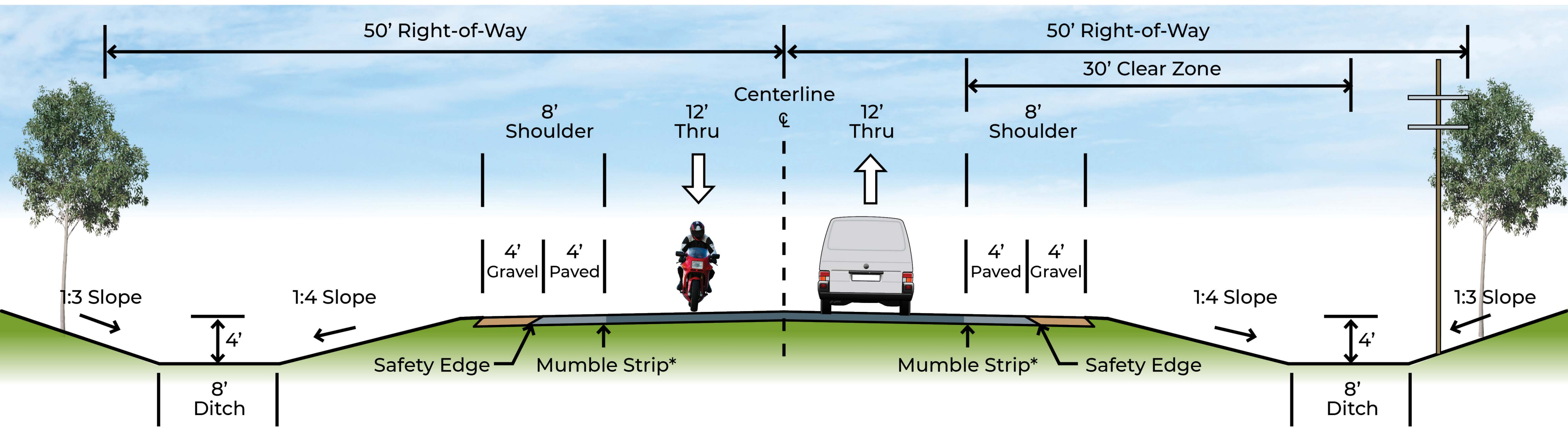
Proposed Highway 40 - Standard Ditch Section
