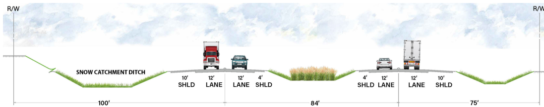
Above drawing shows the recommended four-lane divided highway design with eastbound and westbound lanes separated by a center median ditch and roadside ditches on the outside shoulders of Hwy 212. Turn lanes are included at all public road intersections as well as reduced conflict intersections (RCIs) and a grade separated overpass at Hwy 51.
