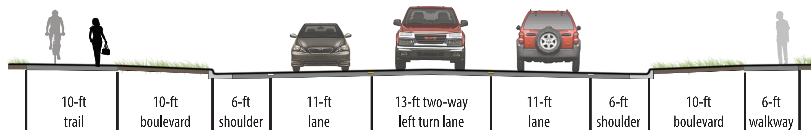
Typical section
