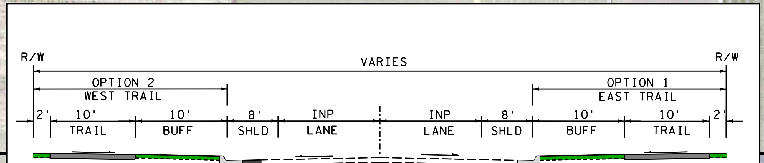
INSET A BAVARIA ROAD URBAN TYPICAL SECTION
